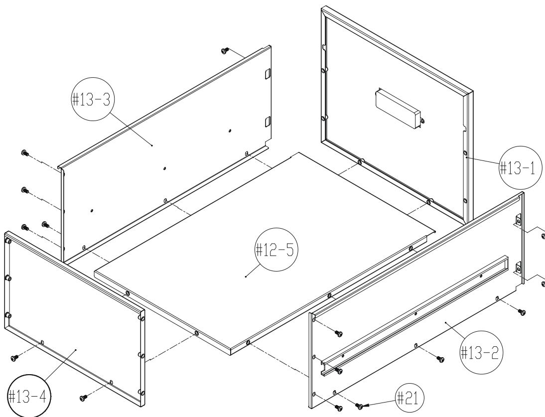
Large Drawer Assembly
