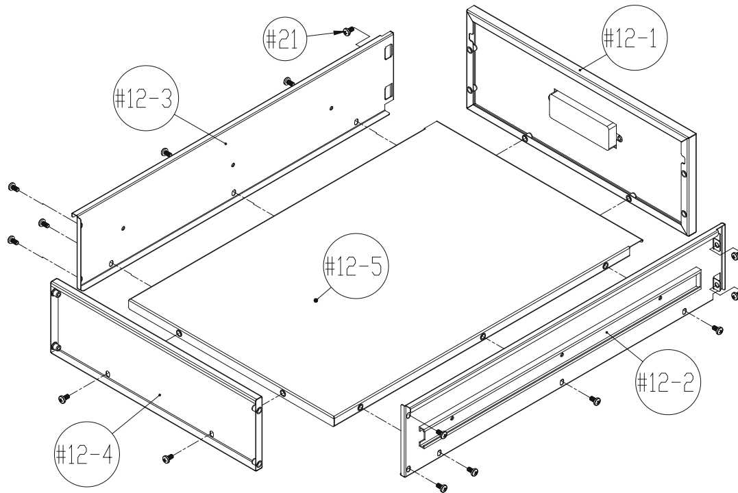
Small Drawer Assembly
